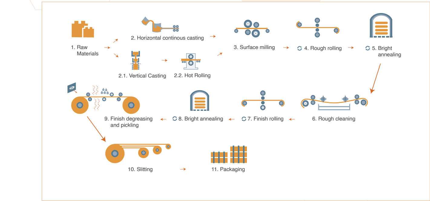
PRODUCTION PROCESS
